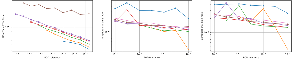
(d) EIM ROM computational times time-only reduction (legend above) (e) ROM computational time time-parameter reduction on parameter and \eta_0 in the training set (legend above) (f) ROM computational time time-parameter reduction on parameter and \eta_0 outside the training set (legend above)
