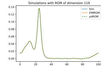
(k) ROM solutions time-parameter reduction with tol_{POD} = 0.001 , N_{RB} = 119 and tol_{EIM} = 0.001 , N_{EIM} = 259 on parameter and \eta_0 in the training set
