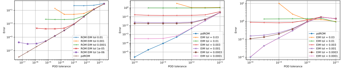
(a) EIM ROM errors time-only reduction (b) ROM errors time-parameter reduction on parameter and \eta_0 in the training set (c) ROM errors time-parameter reduction on parameter and \eta_0 outside the training set
