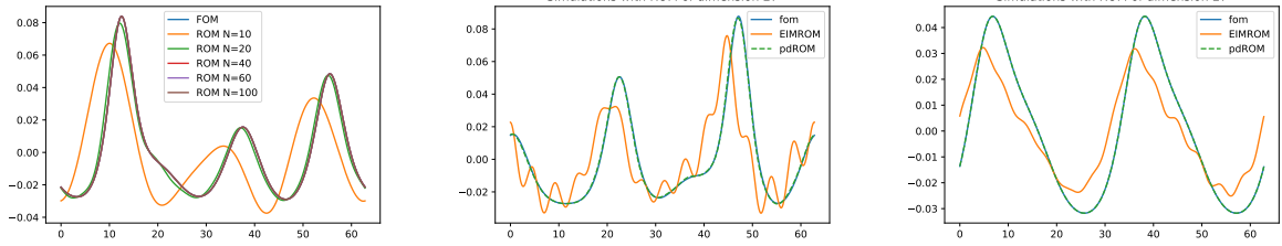
(g) ROM solutions time-only reduction (h) ROM solutions time-parameter reduction with tol_{POD} = 0.3 , N_{RB} = 27 and tol_{EIM} = 0.03 , N_{EIM} = 72 on parameter and \eta_0 in the training set (i) ROM solutions time-parameter reduction with N_{RB} = 27 and N_{EIM} = 72 on parameter and \eta_0 outside the training set
