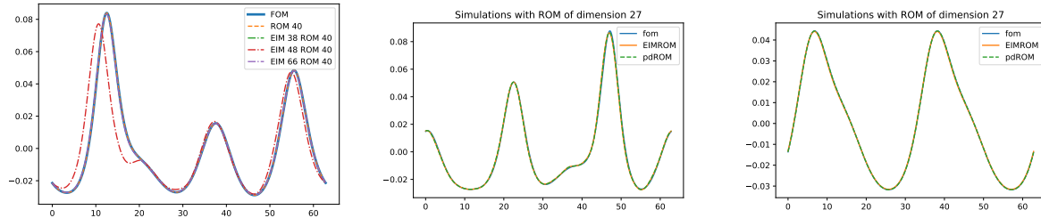
(j) ROM solutions time-only reduction (k) ROM solutions time-parameter reduction with tol_{POD} = 0.3 , N_{RB} = 27 and tol_{EIM} = 0.0003 , N_{EIM} = 119 on parameter and \eta_0 in the training set (l) ROM solutions time-parameter reduction with N_{RB} = 27 and N_{EIM} = 119 on parameter and \eta_0 outside the training set
