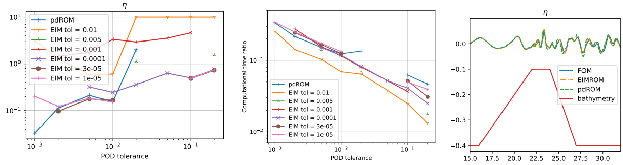
(a) ROM errors time-parameter reduction on parameter outside the training set (b) ROM computational time time-parameter reduction on parameter and u_0 outside the training set (c) pdROM and EIMROM solutions time-parameter reduction
