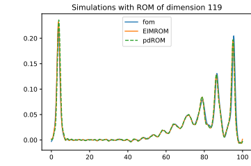
(l) ROM solutions time-parameter reduction with tol_{POD} = 0.001 , N_{RB} = 119 and tol_{EIM} = 0.001 , N_{EIM} = 259 on parameter and \eta_0 outside the training set
