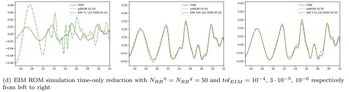
Figure 15: Monochromatic waves on a submerged bar. pdROM and EIM (time-only) reduction: simulation, errors and computational time, varying POD and EIM dimensions
